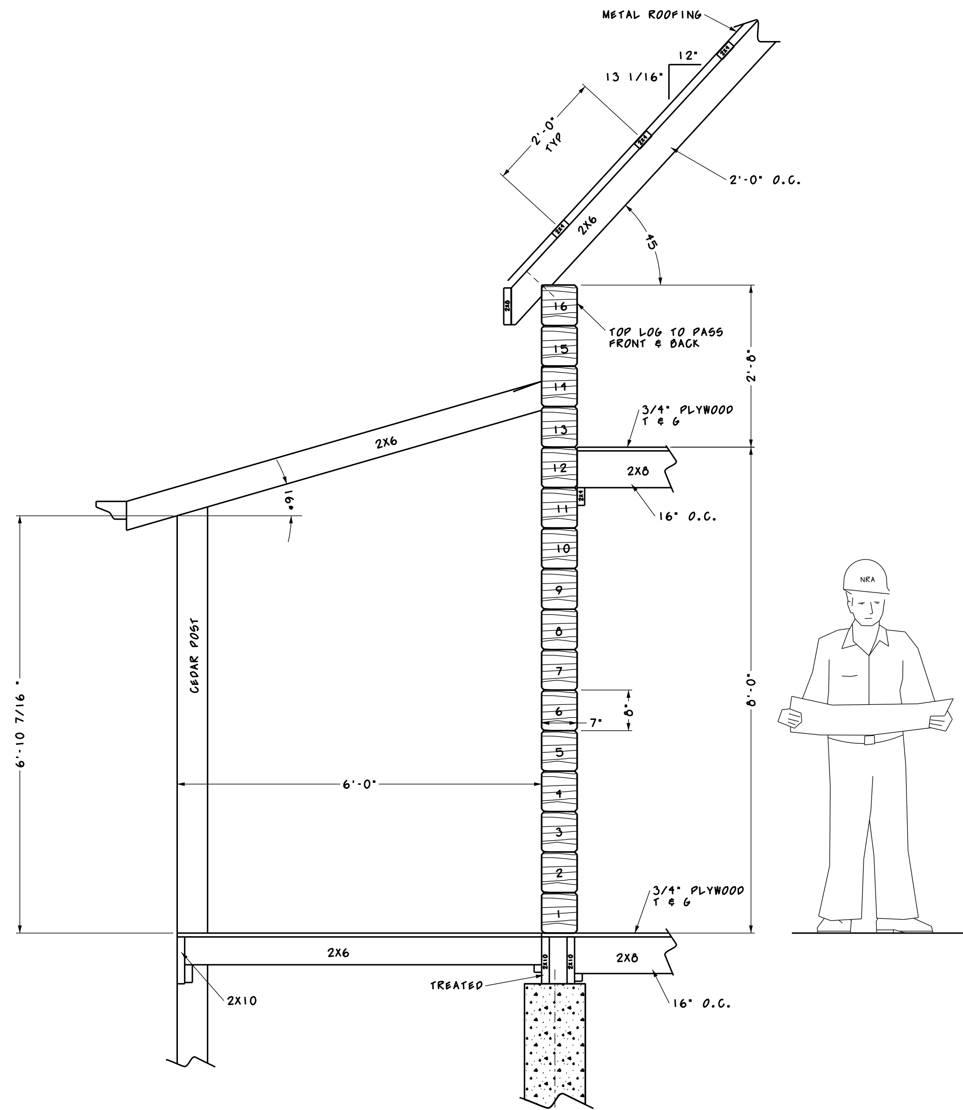
WALL SECTION
